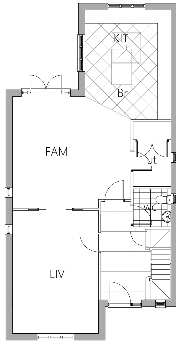
GROUND FLOOR AS PROPOSED
